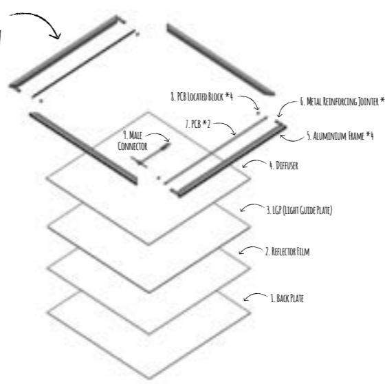
LED PANEL EXPLODED VIEW
