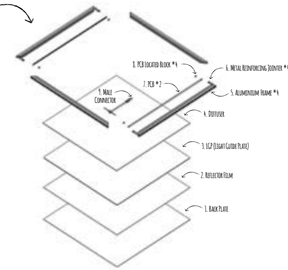
LED PANEL EXPLODED VIEW
